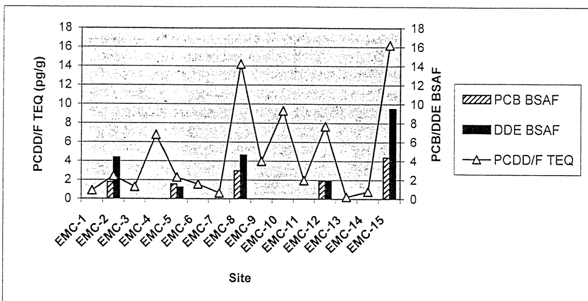
FIGURE 5. DDE and PCB BSAFs, and PCDD/F TEQs in surficial composite and discrete sediment samples collected from the AOC.
